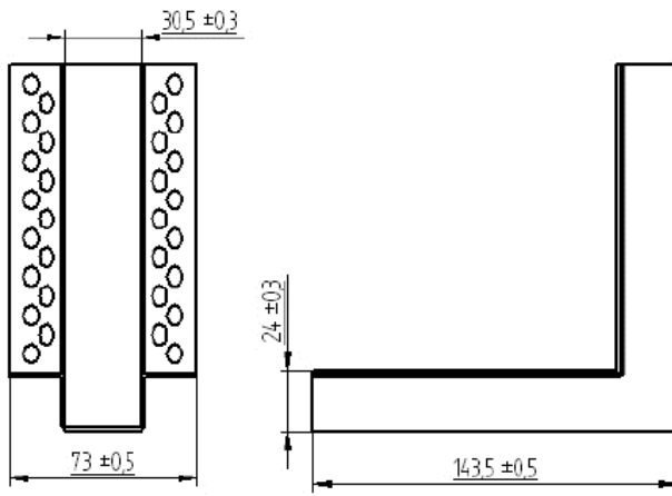
Fig. 13. Corner bead BP11 K H3 WEW
