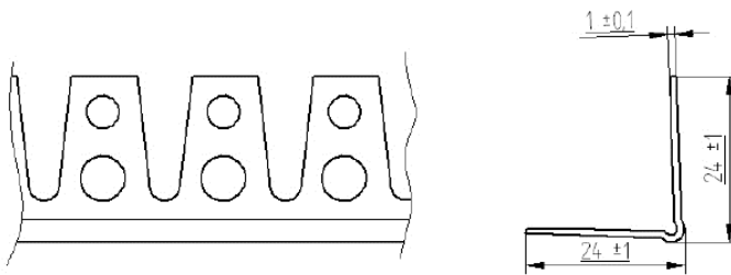
Fig. 17. Corner bead BP3
