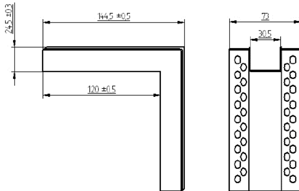
Fig. 13. Corner bead BP11 K H3 WEW
