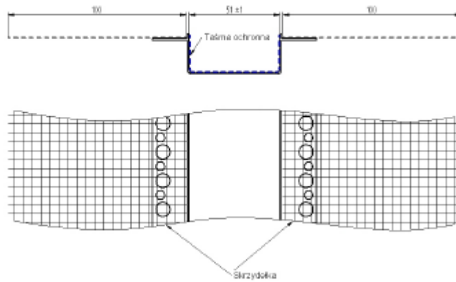
Fig. 6. Beads BP11 H1S (a), BP11 H2S (b), BP11 H3S (c), BP11 H3 NS (d), BP11 H5S (e) cont.
