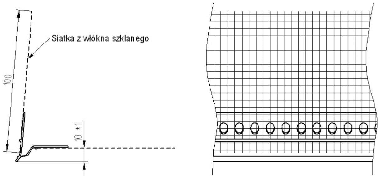
Fig. 2. Bead BP14 LUX
