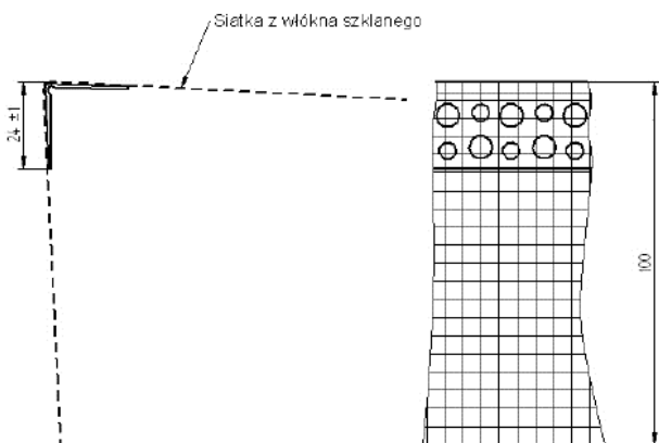
Fig. 5. Corner bead BP10
